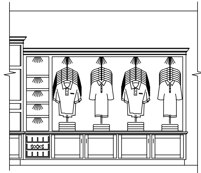
5 ELEVATION - 1/2" = 1'-0"
