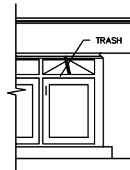
13 ELEVATION 1/2" = 1'-0"
