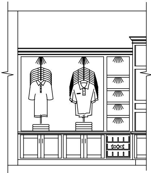
3 ELEVATION - 1/2" = 1'-0"
