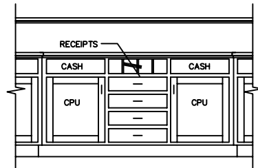
12 ELEVATION 1/2" = 1'-0"
