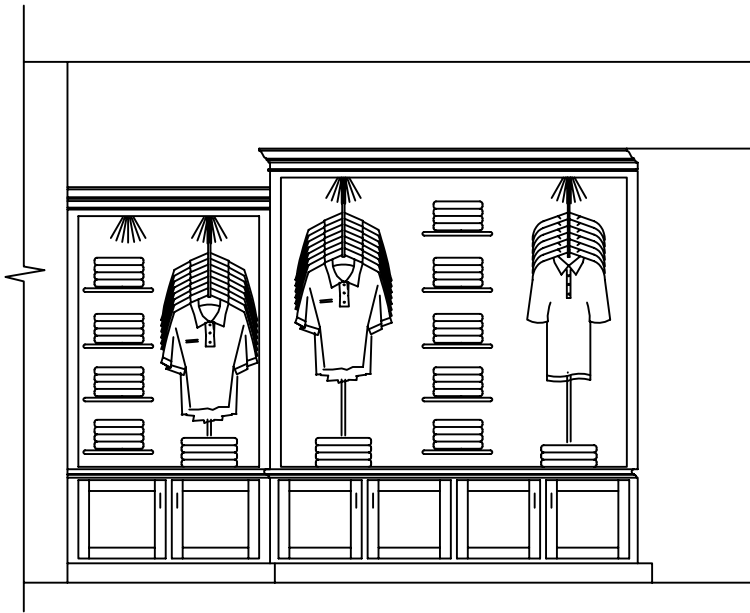
1 ELEVATION - 1/2" = 1'-0"
