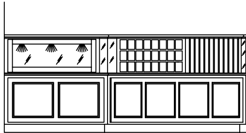
6 ELEVATION 1/2" = 1'-0"
